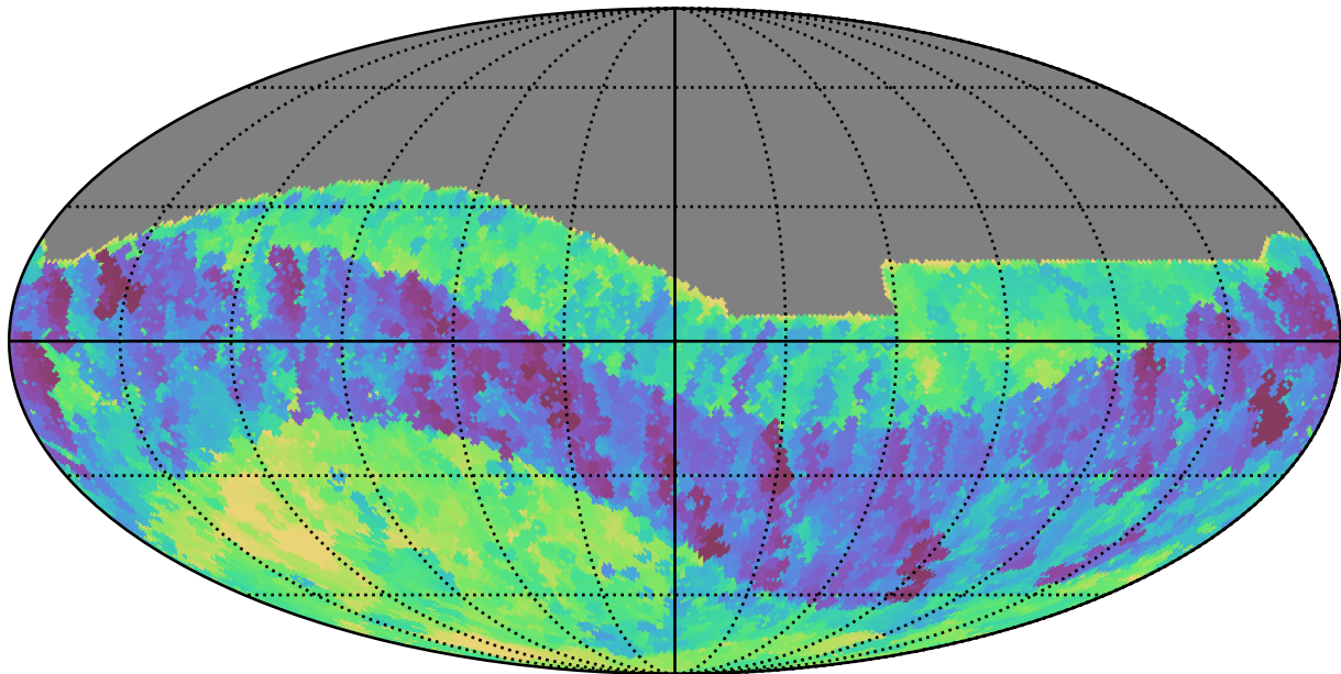
too_10_4v3.4_10yrs All sky z band: Min fiveSigmaDepth
