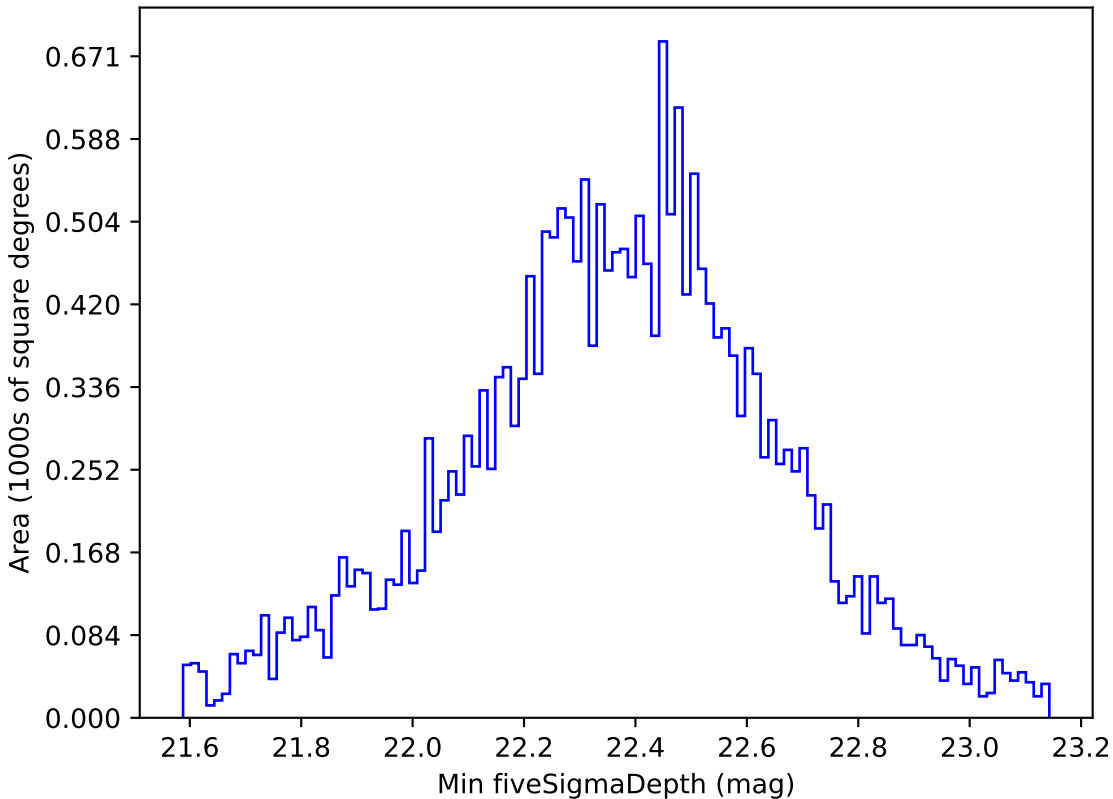
too_10_4v3.4_10yrs All sky u band: Min fiveSigmaDepth
