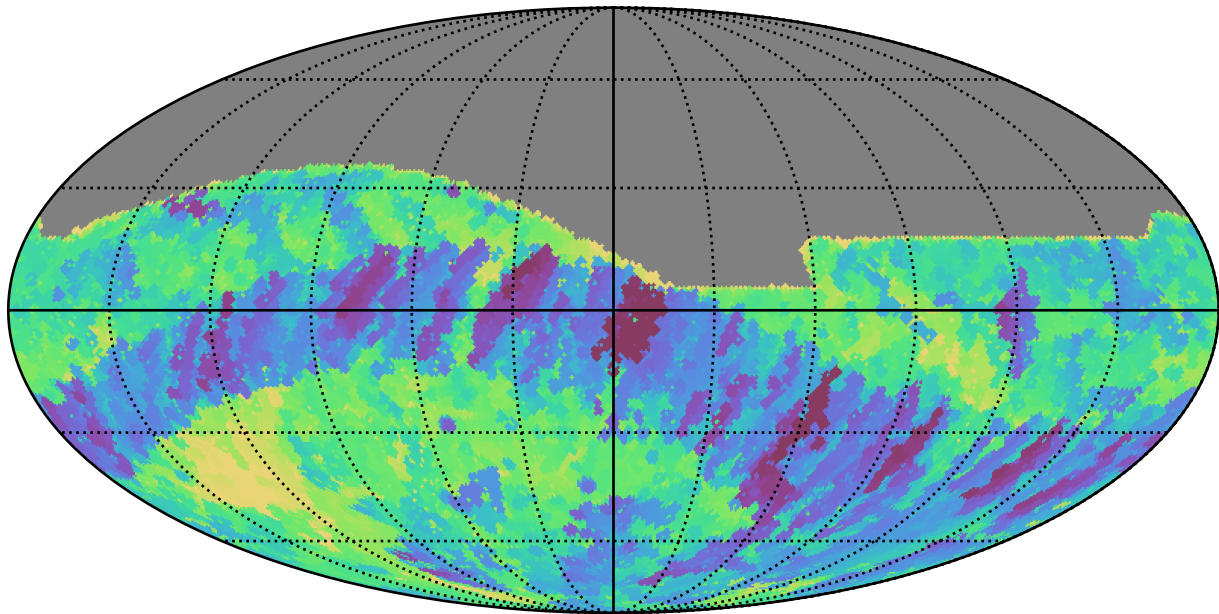
too_10_4v3.4_10yrs All sky r band: Min fiveSigmaDepth
