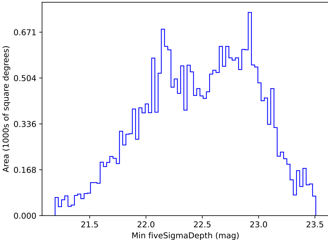
too_10_4v3.4_10yrs All sky r band: Min fiveSigmaDepth
