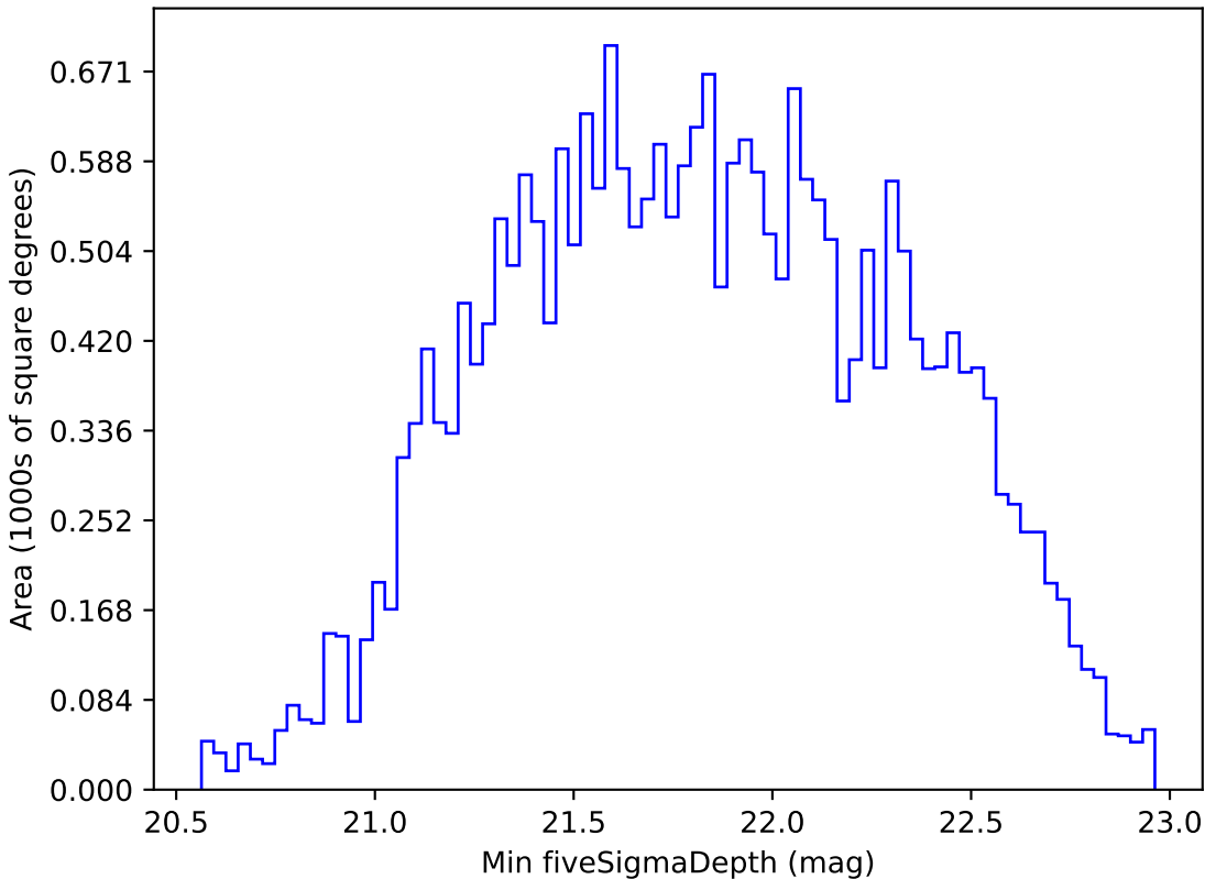
too_10_4v3.4_10yrs All sky i band: Min fiveSigmaDepth
