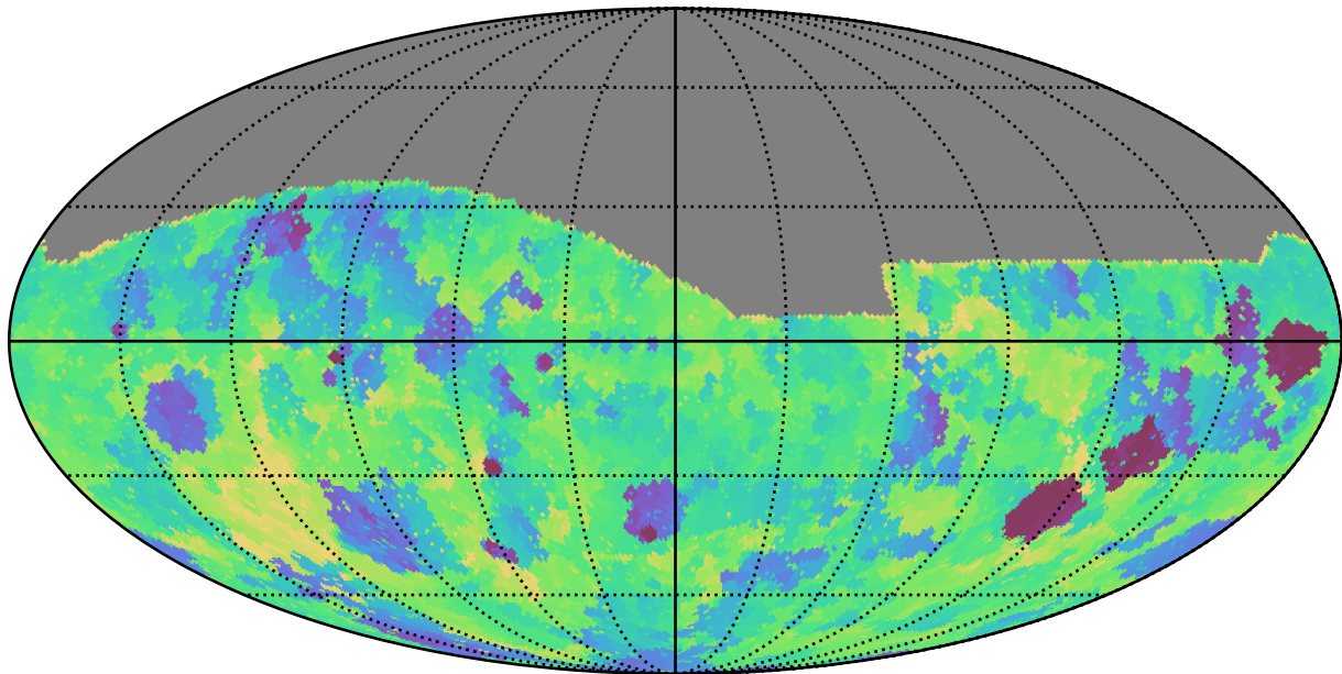
too_10_4v3.4_10yrs All sky g band: Min fiveSigmaDepth
