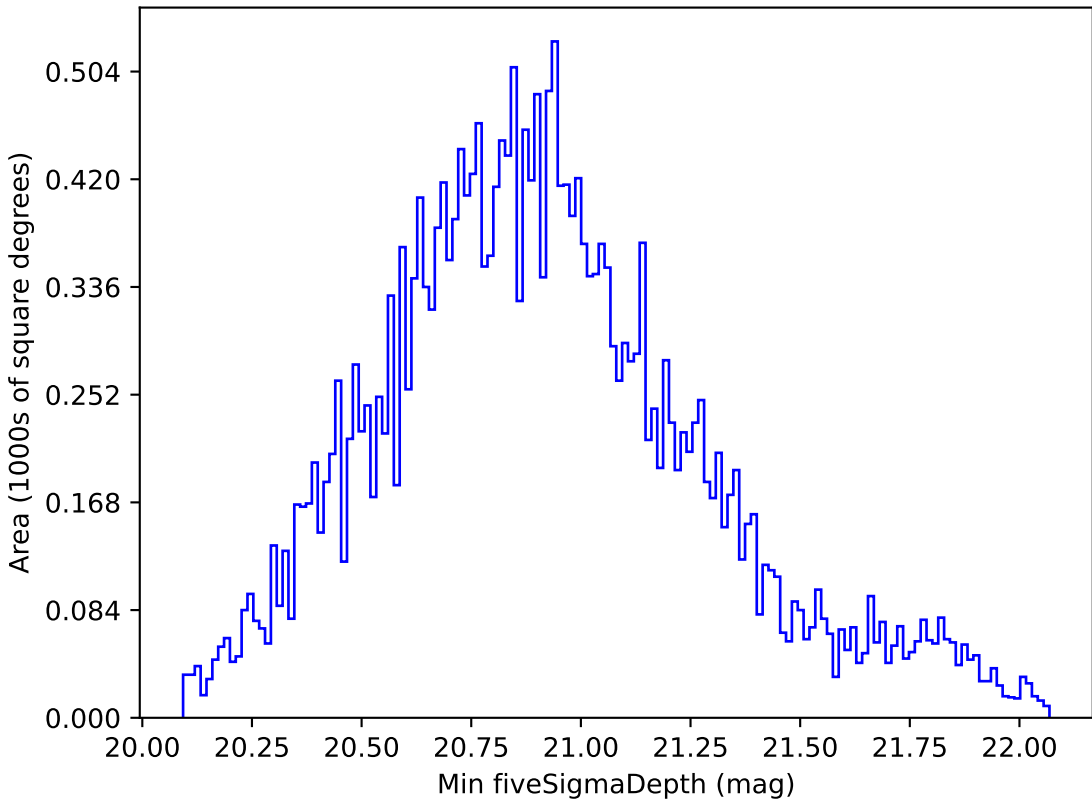
too_10_4v3.4_10yrs All sky all bands: Min fiveSigmaDepth
