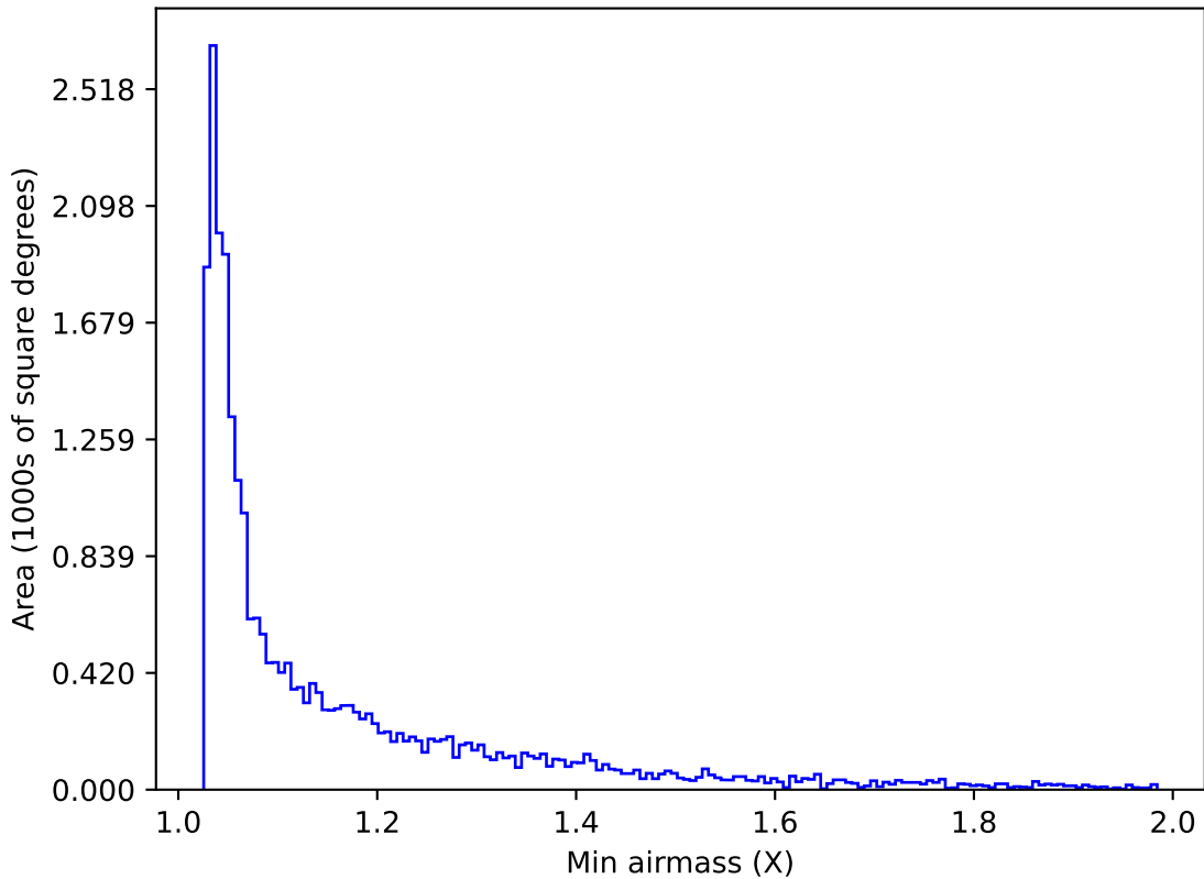
too_10_4v3.4_10yrs Yr 1 z band: Min airmass
