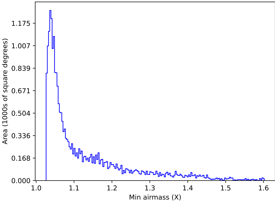
too_10_4v3.4_10yrs Yr 1 y band: Min airmass
