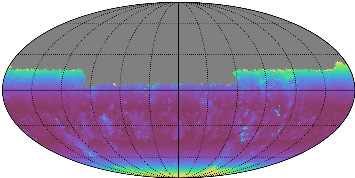
too_10_4v3.4_10yrs Yr 1 u band: Min airmass
