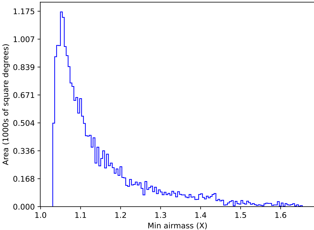
too_10_4v3.4_10yrs Yr 1 u band: Min airmass
