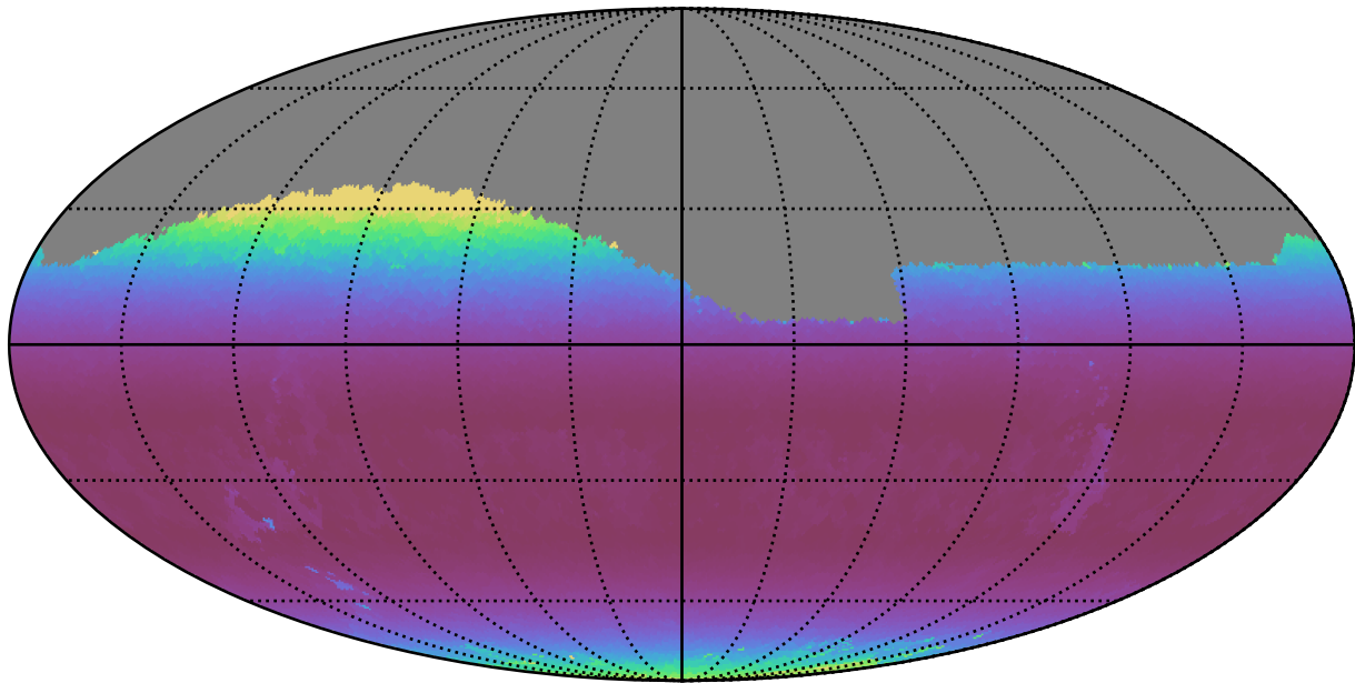
too_10_4v3.4_10yrs Yr 1 i band: Min airmass
