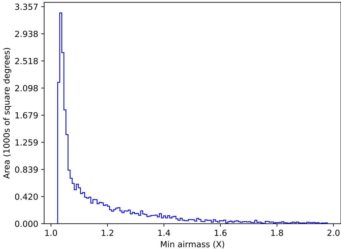
too_10_4v3.4_10yrs Yr 1 i band: Min airmass
