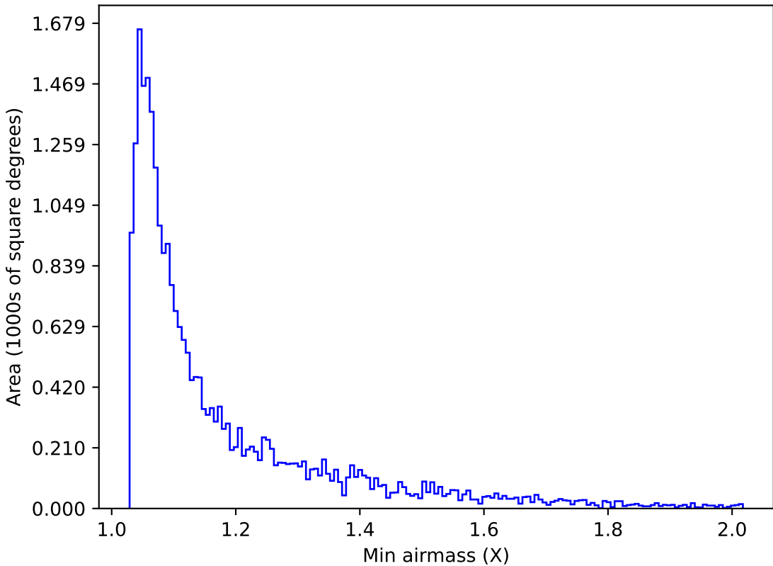
too_10_4v3.4_10yrs Yr 1 g band: Min airmass
