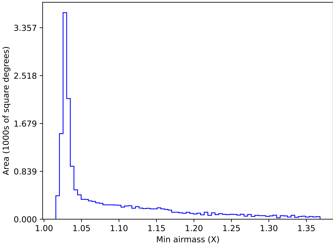
too_10_4v3.4_10yrs WFD z band: Min airmass
