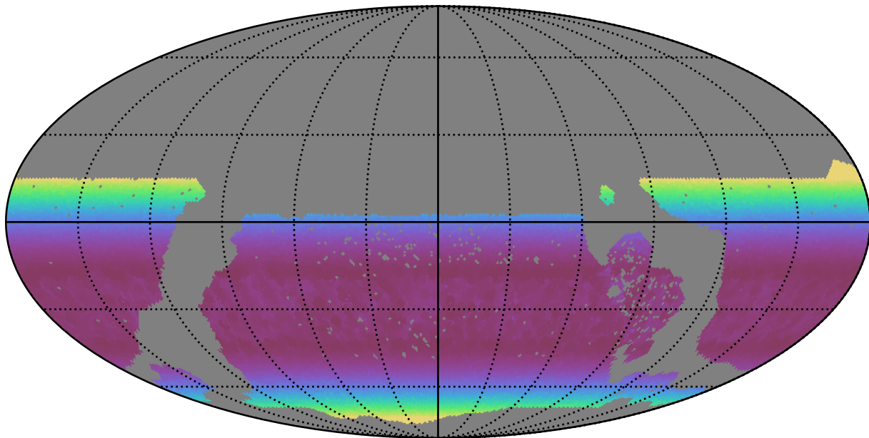
too_10_4v3.4_10yrs WFD u band: Min airmass
