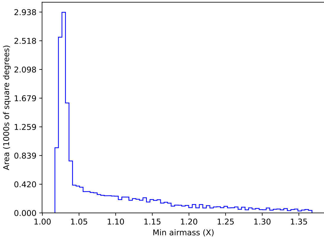
too_10_4v3.4_10yrs WFD r band: Min airmass
