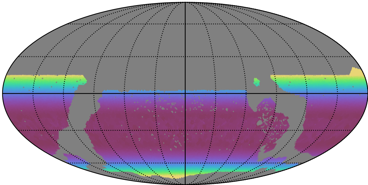
too_10_4v3.4_10yrs WFD i band: Min airmass
