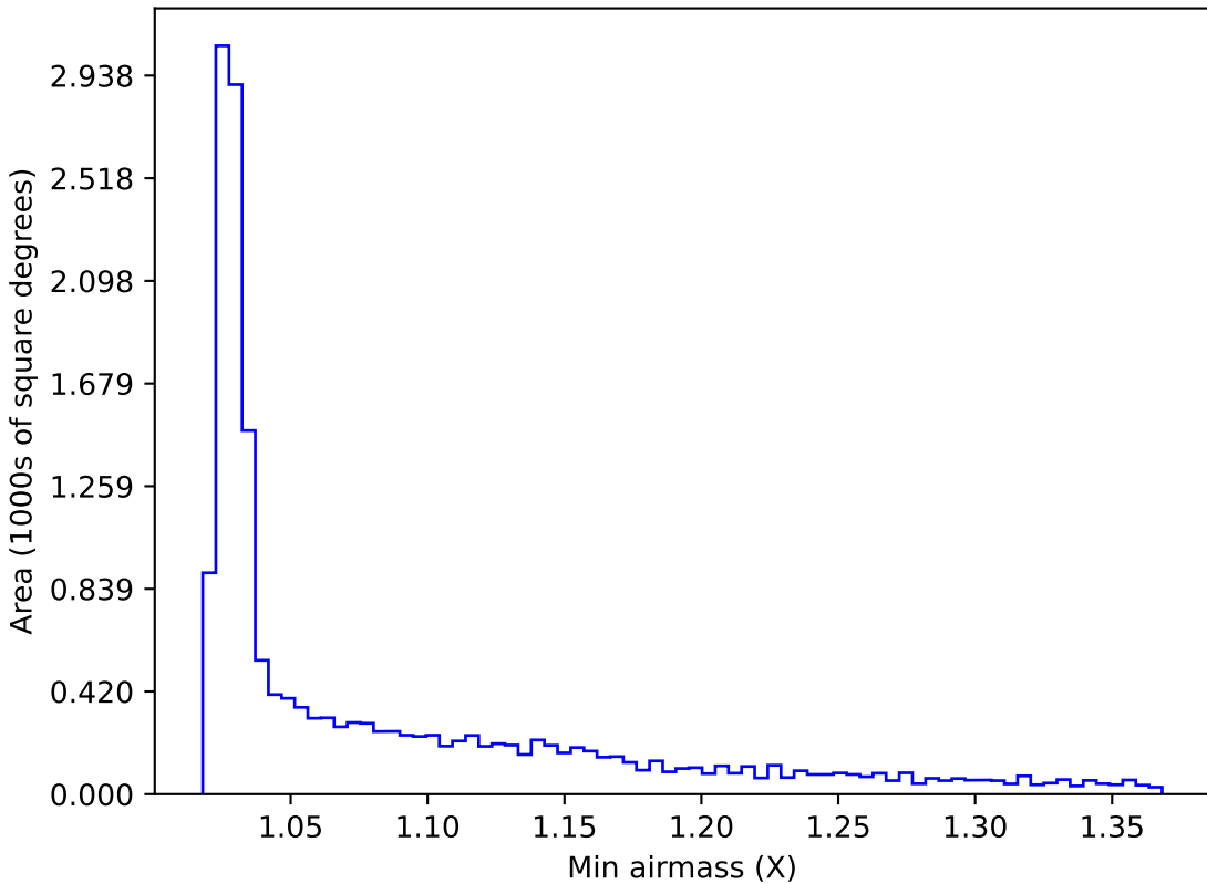
too_10_4v3.4_10yrs WFD i band: Min airmass
