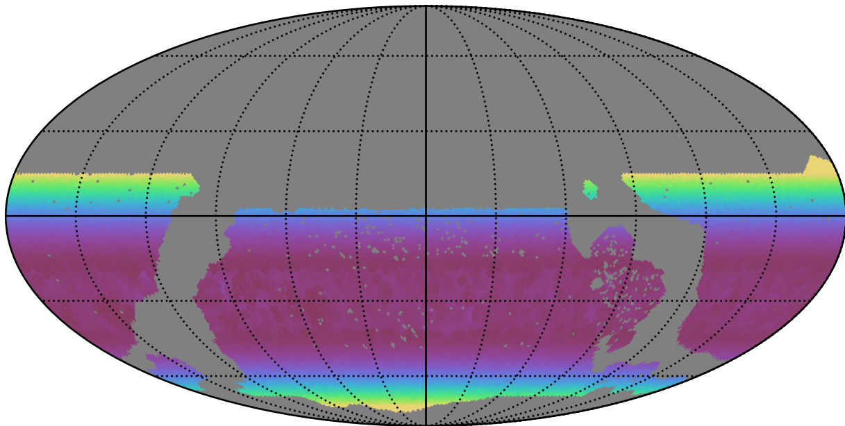
too_10_4v3.4_10yrs WFD g band: Min airmass
