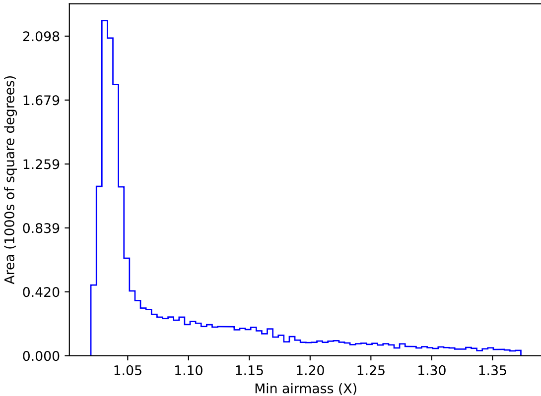
too_10_4v3.4_10yrs WFD g band: Min airmass
