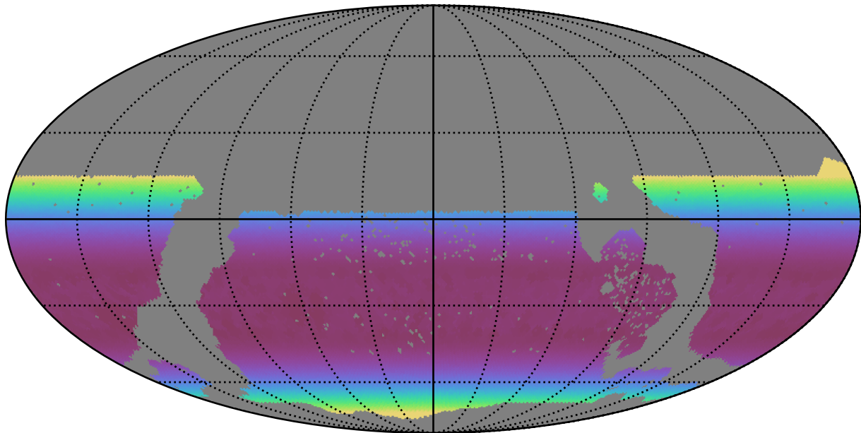
too_10_4v3.4_10yrs WFD all bands: Min airmass
