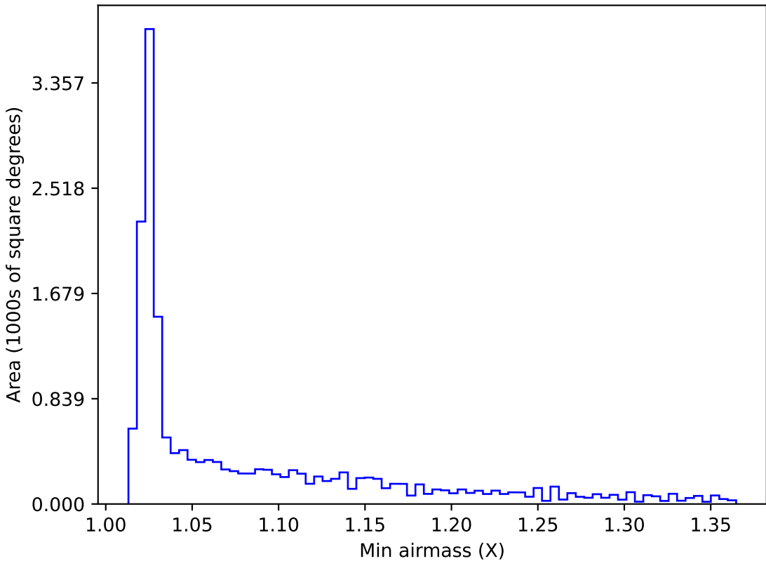
too_10_4v3.4_10yrs WFD all bands: Min airmass
