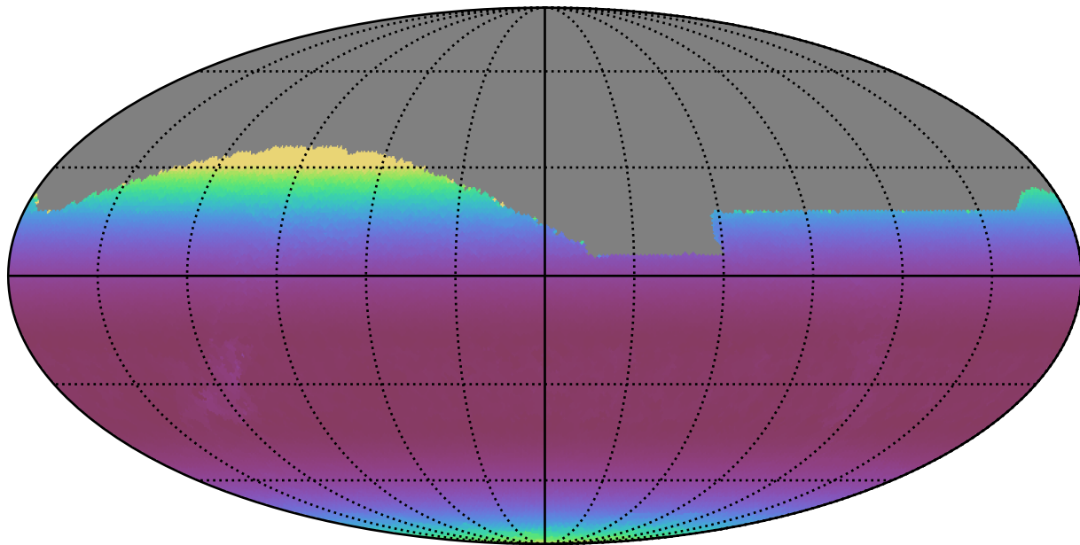
too_10_4v3.4_10yrs All sky z band: Min airmass
