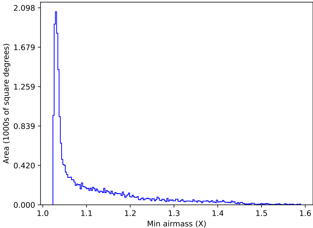
too_10_4v3.4_10yrs All sky y band: Min airmass
