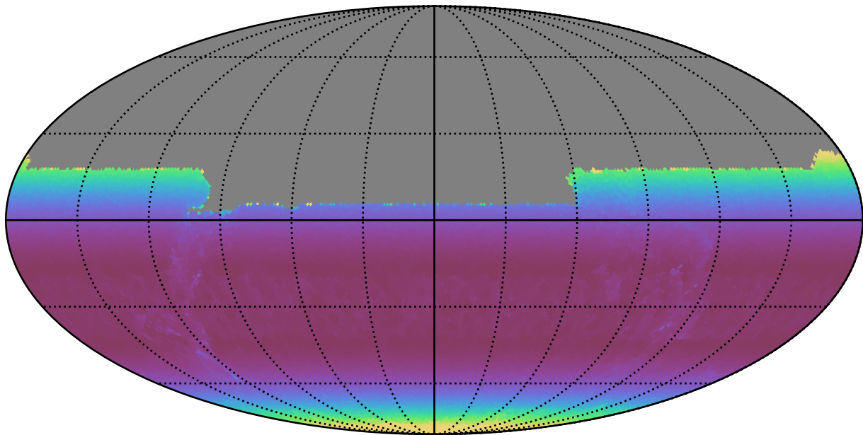
too_10_4v3.4_10yrs All sky u band: Min airmass
