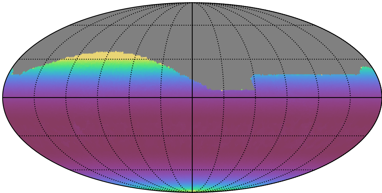
too_10_4v3.4_10yrs All sky r band: Min airmass
