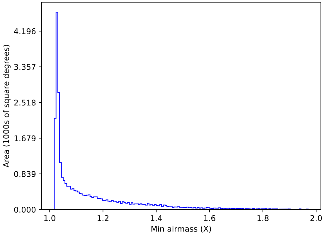
too_10_4v3.4_10yrs All sky r band: Min airmass
