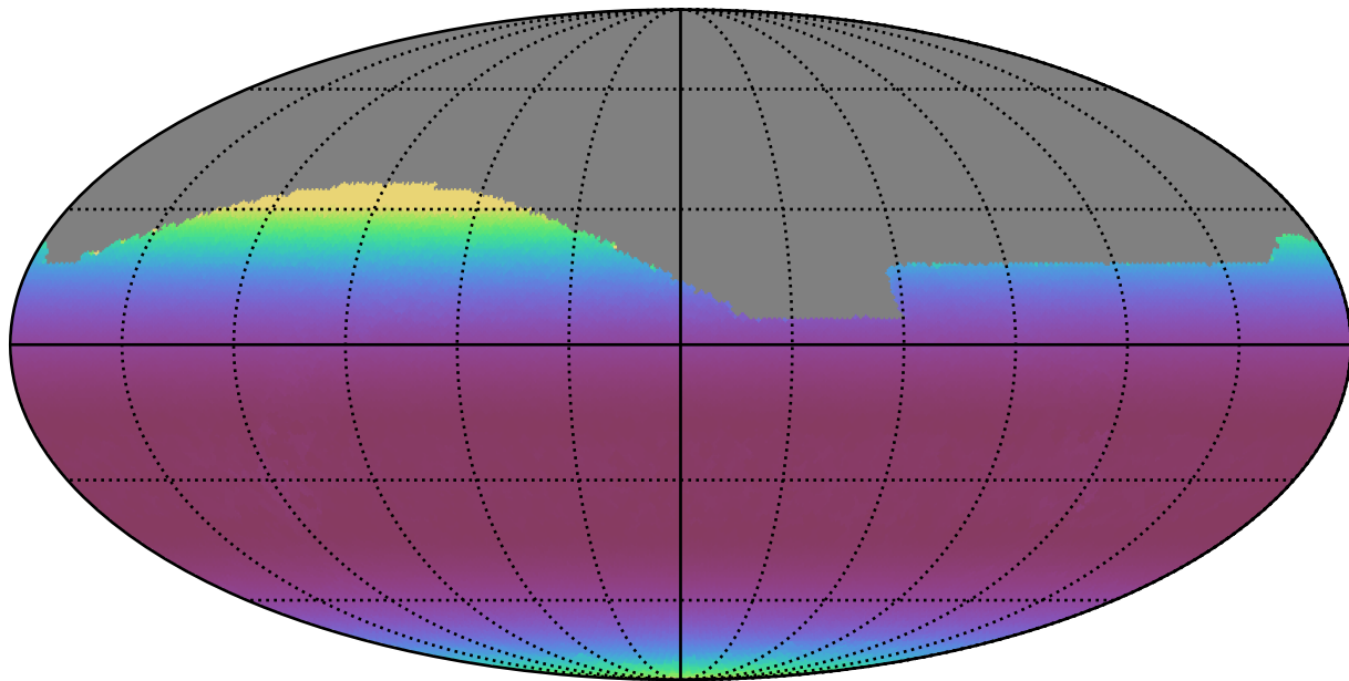
too_10_4v3.4_10yrs All sky i band: Min airmass
