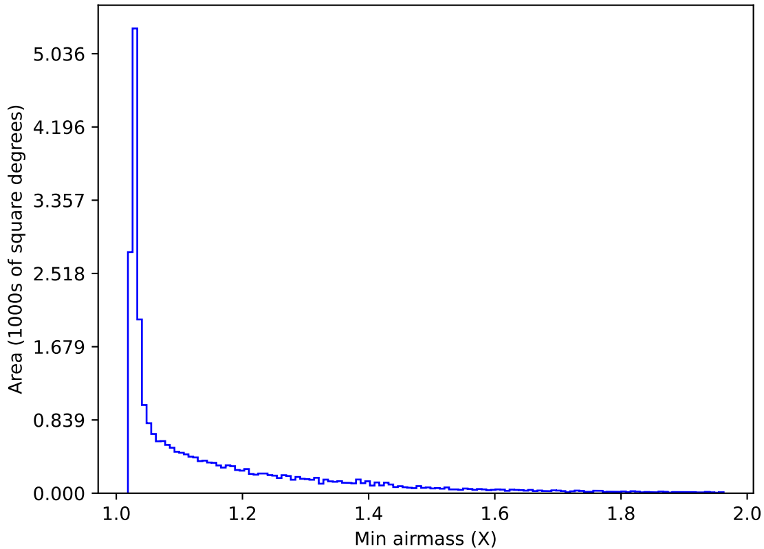
too_10_4v3.4_10yrs All sky i band: Min airmass
