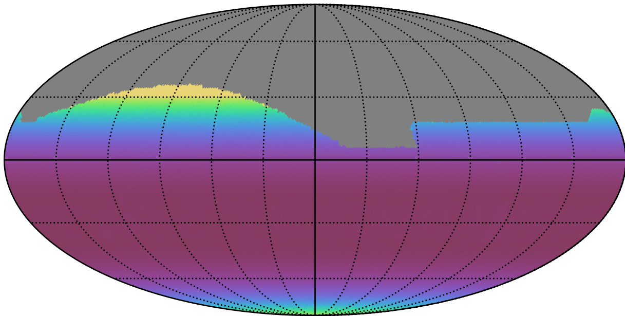
too_10_4v3.4_10yrs All sky all bands: Min airmass
