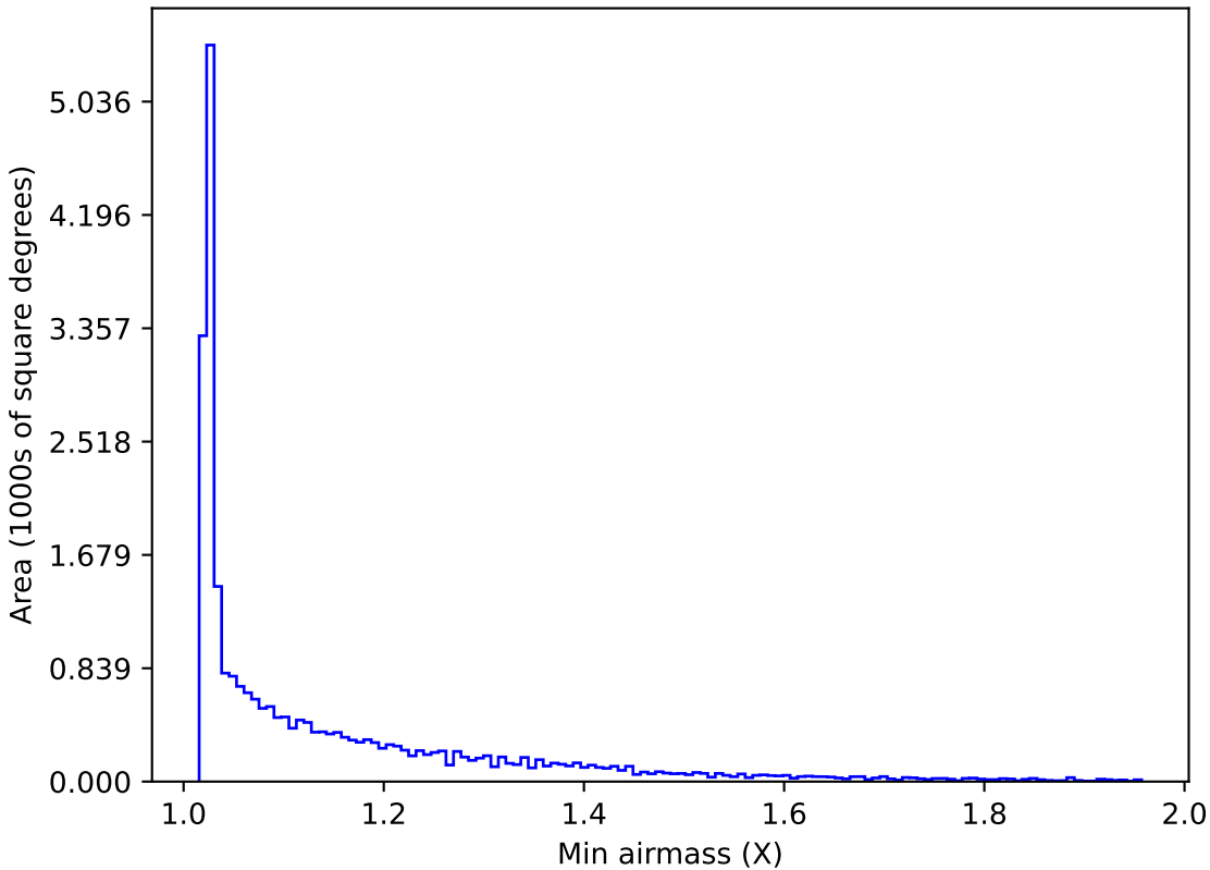
too_10_4v3.4_10yrs All sky all bands: Min airmass
