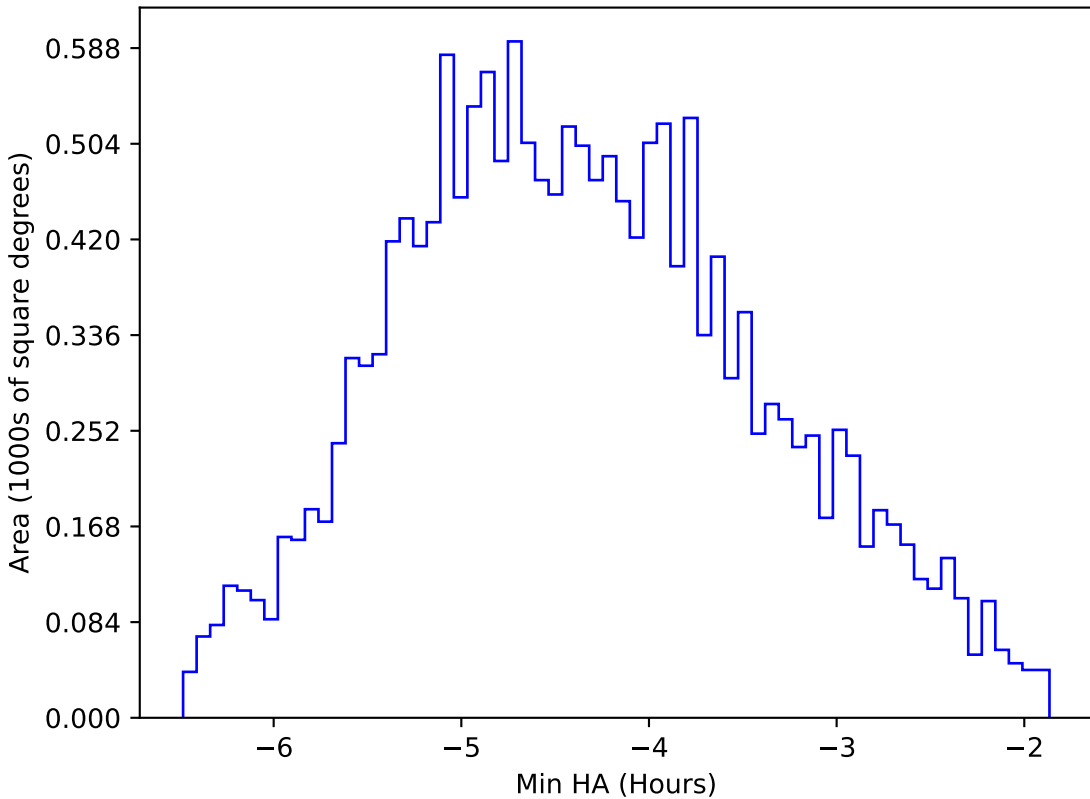
too_10_4v3.4_10yrs WFD z band: Min HA
