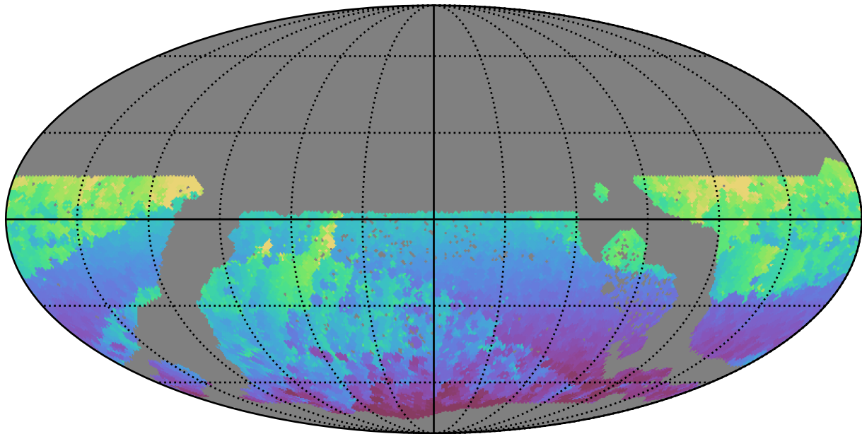
too_10_4v3.4_10yrs WFD r band: Min HA
