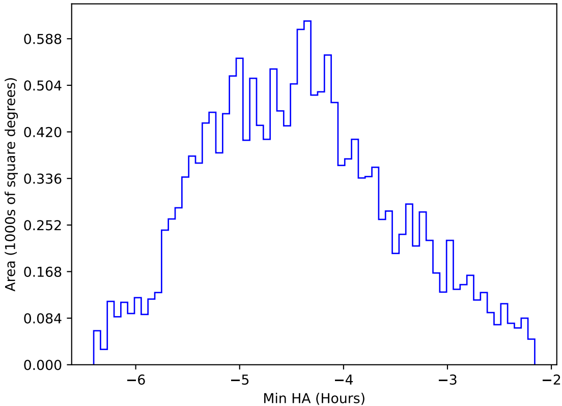
too_10_4v3.4_10yrs WFD r band: Min HA
