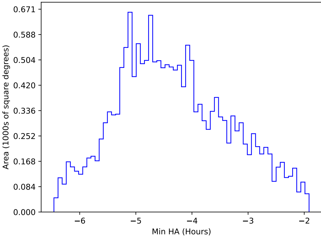
too_10_4v3.4_10yrs WFD i band: Min HA
