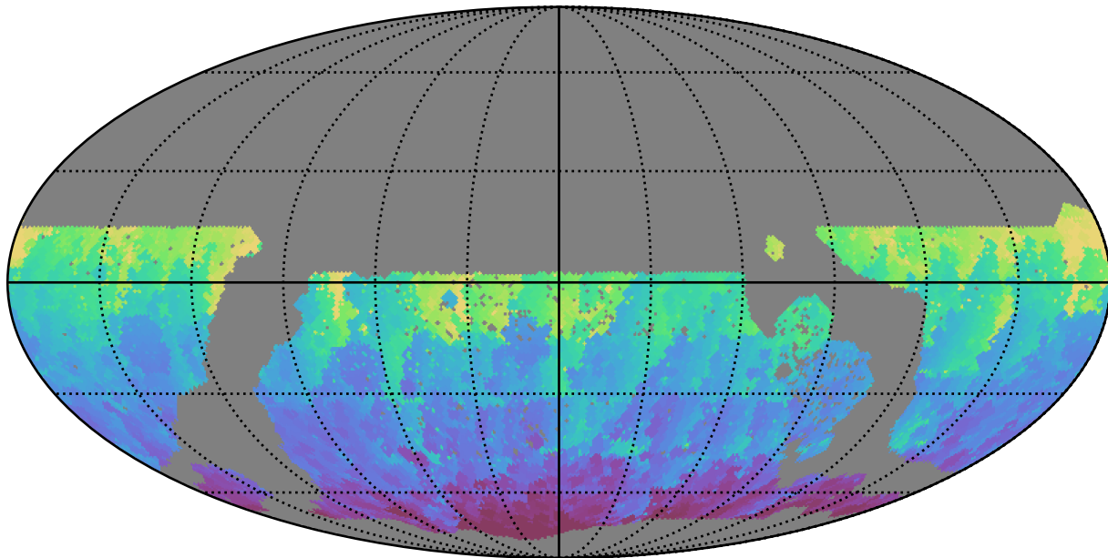
too_10_4v3.4_10yrs WFD g band: Min HA
