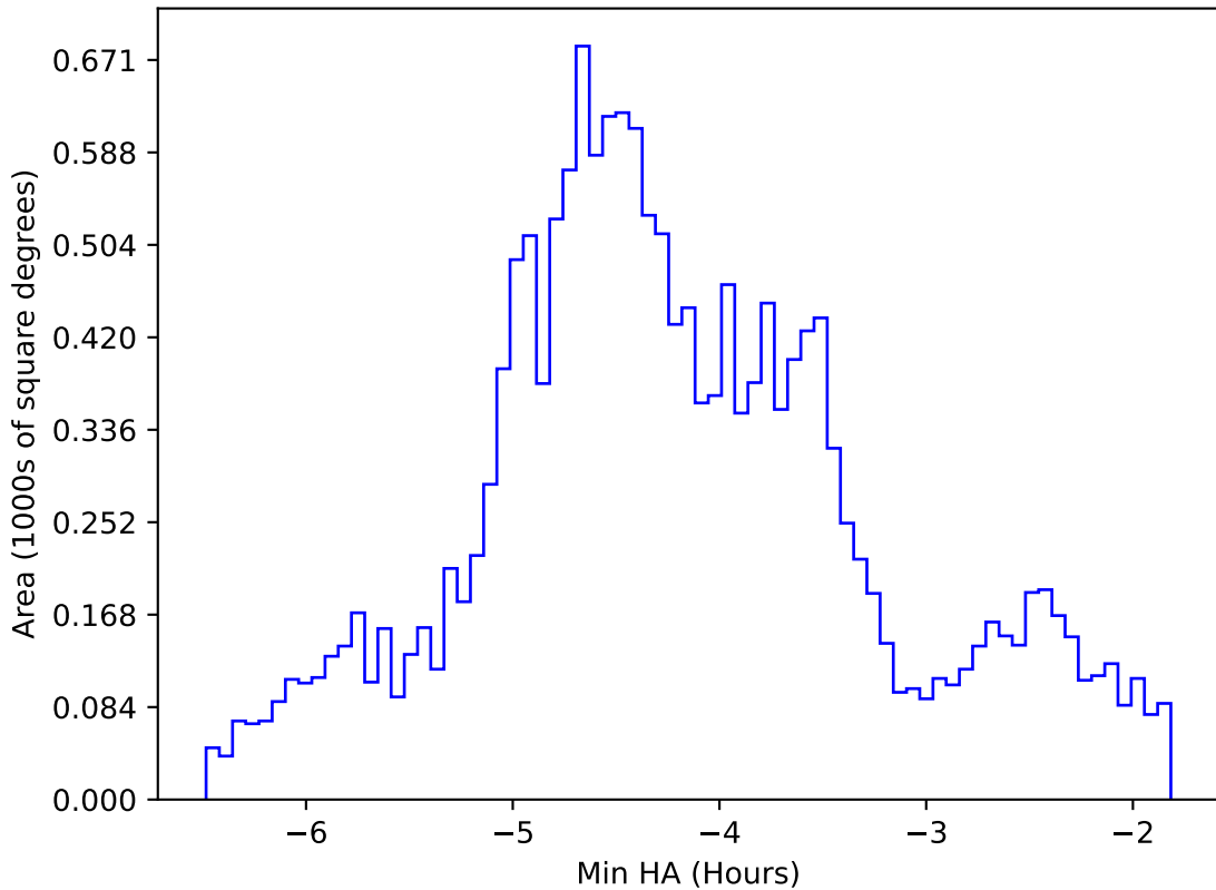
too_10_4v3.4_10yrs WFD g band: Min HA
