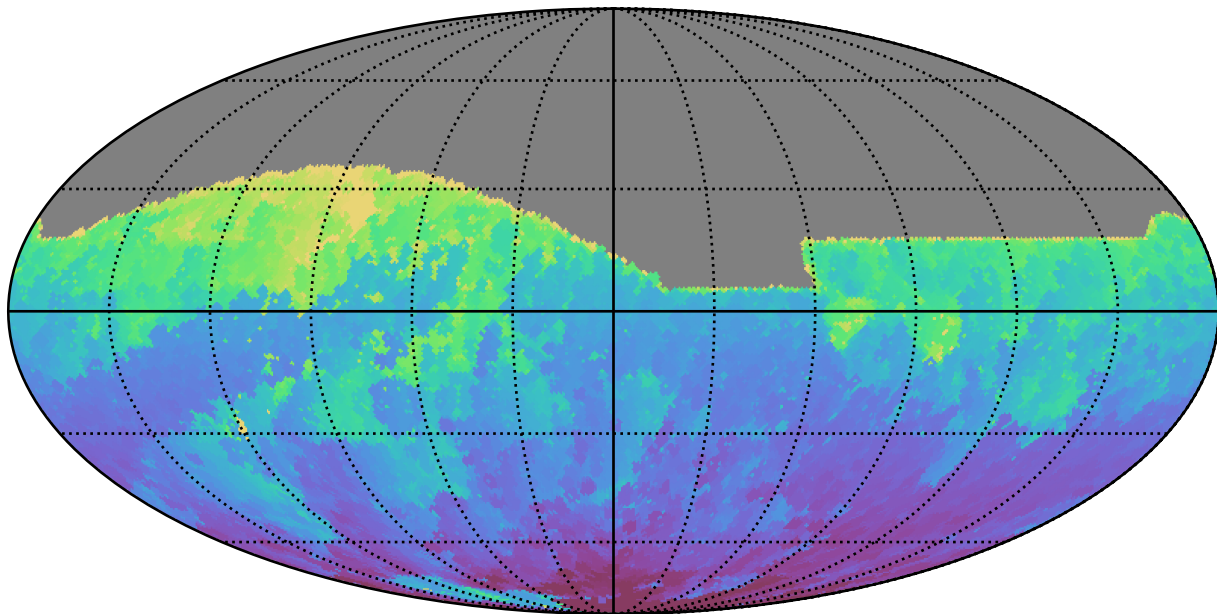
too_10_4v3.4_10yrs All sky z band: Min HA
