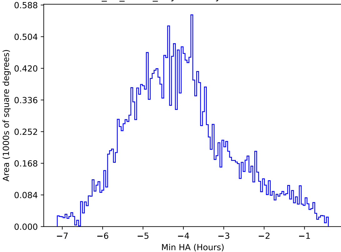
too_10_4v3.4_10yrs All sky z band: Min HA
