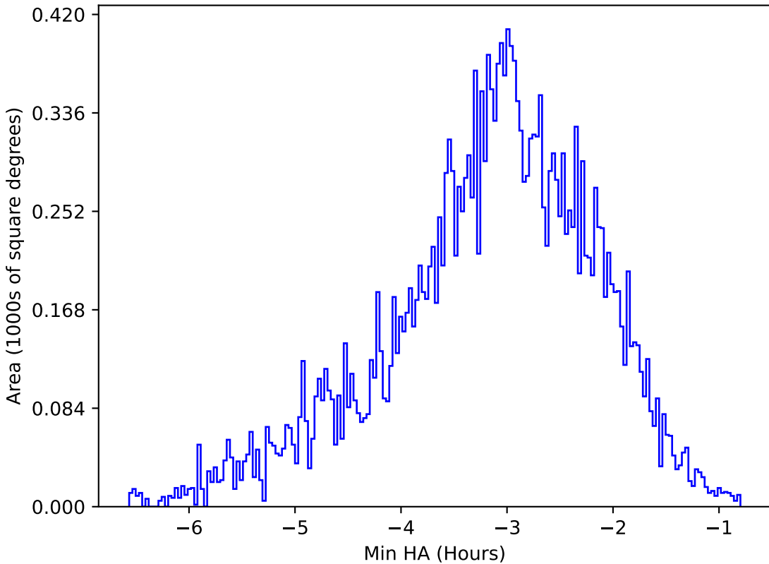
too_10_4v3.4_10yrs All sky u band: Min HA
