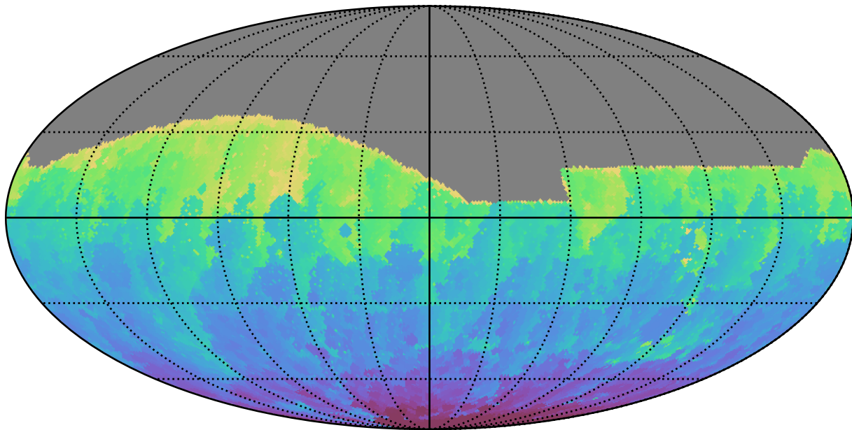
too_10_4v3.4_10yrs All sky g band: Min HA
