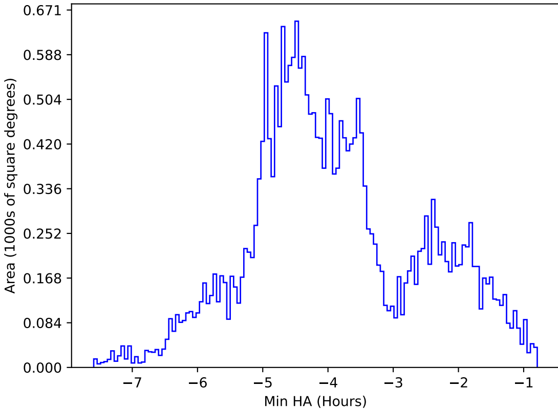
too_10_4v3.4_10yrs All sky g band: Min HA
