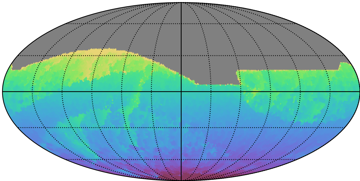
too_10_4v3.4_10yrs All sky all bands: Min HA
