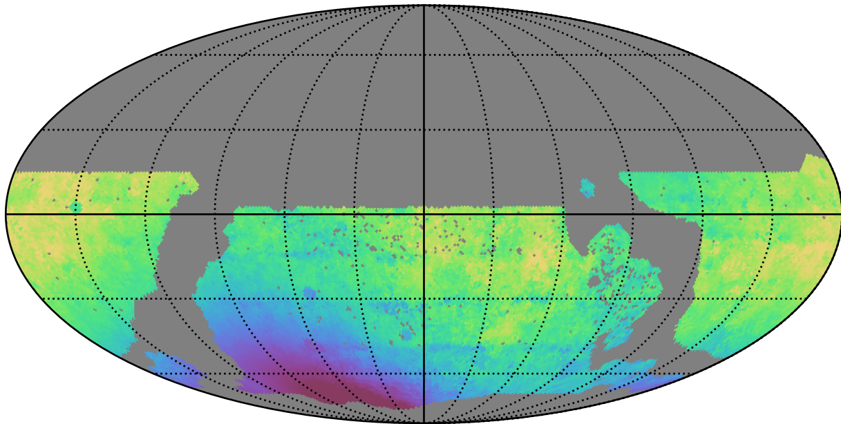
too_10_4v3.4_10yrs WFD z band: Median solarElong
