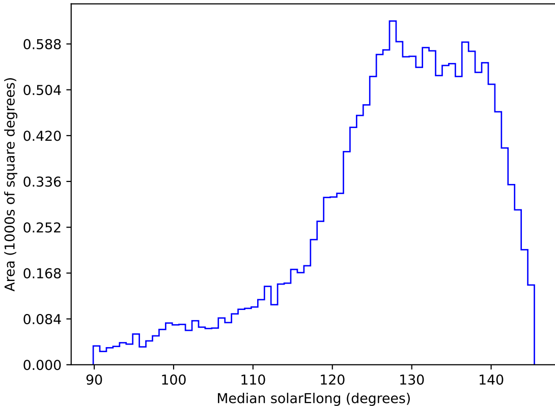
too_10_4v3.4_10yrs WFD z band: Median solarElong
