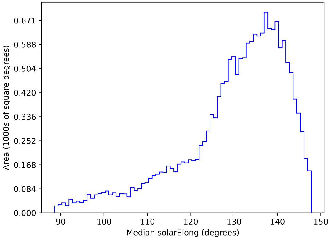
too_10_4v3.4_10yrs WFD y band: Median solarElong
