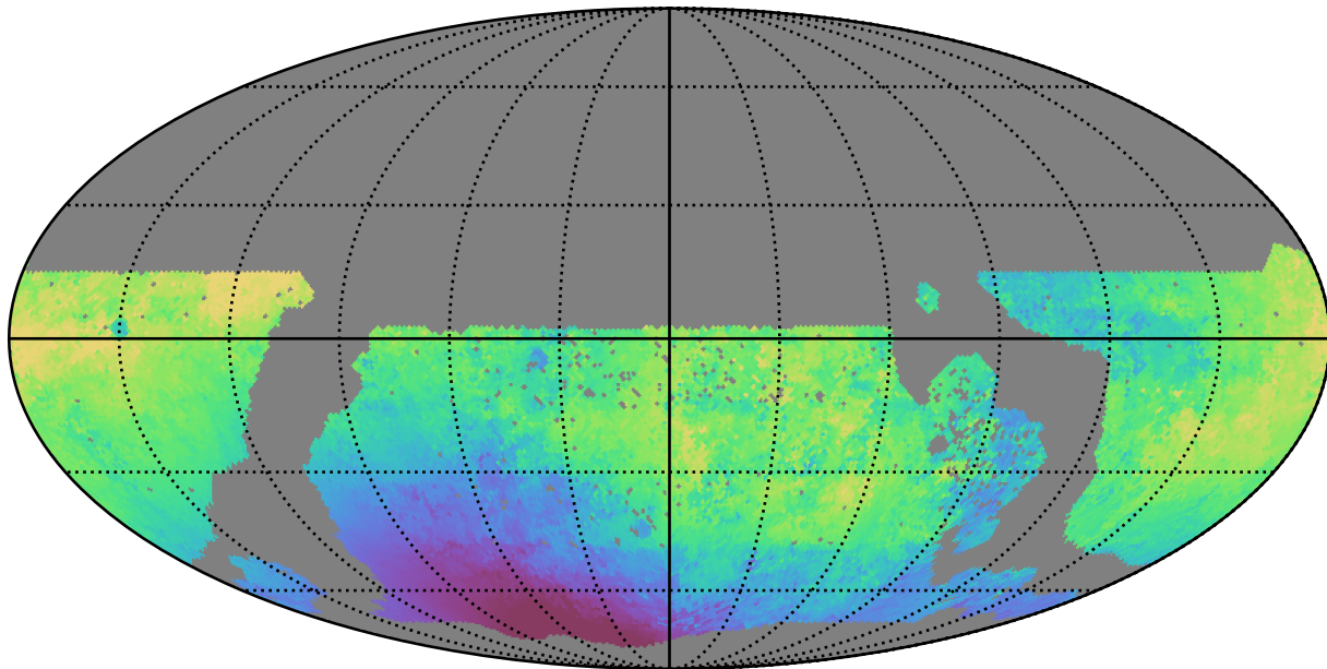
too_10_4v3.4_10yrs WFD u band: Median solarElong
