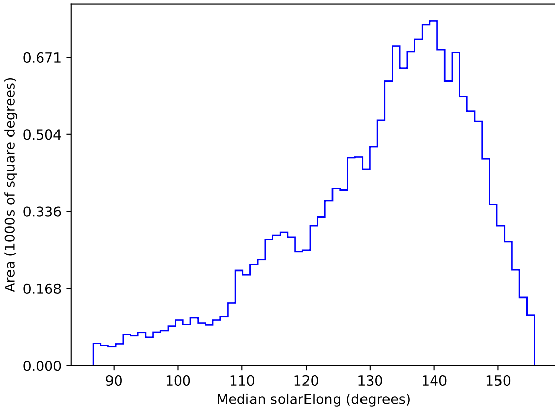
too_10_4v3.4_10yrs WFD u band: Median solarElong
