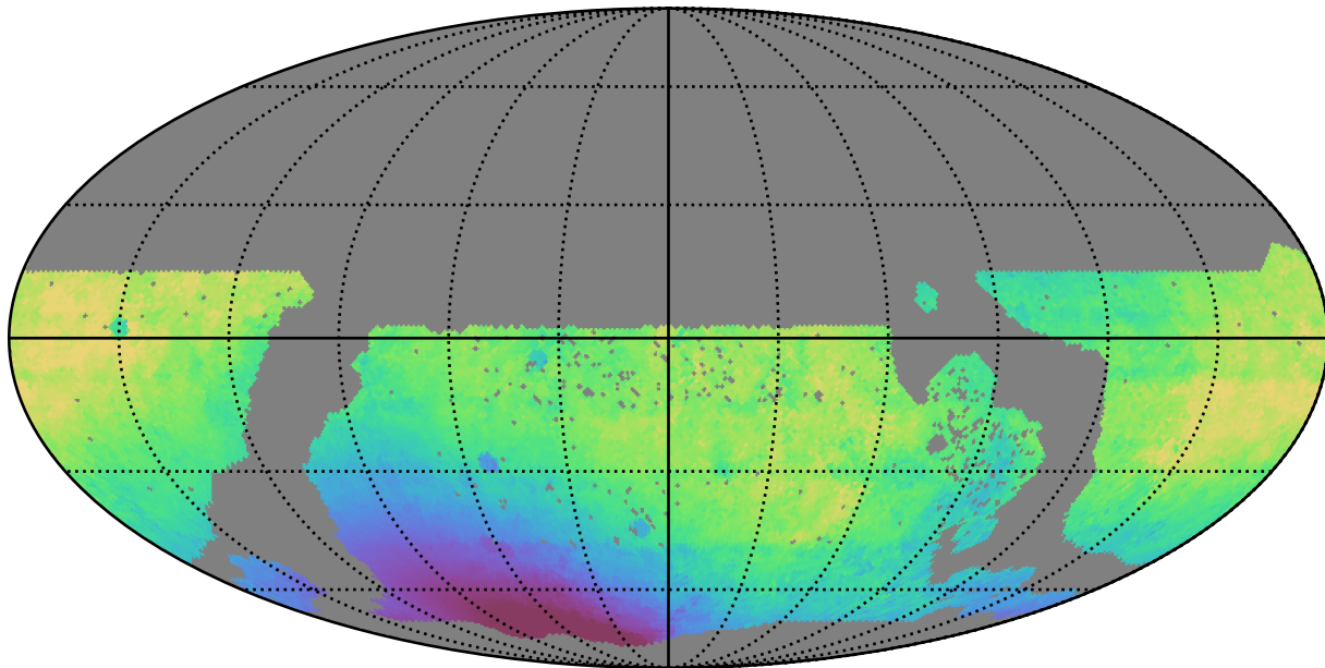
too_10_4v3.4_10yrs WFD r band: Median solarElong
